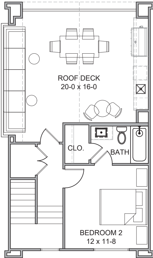
FOURTH FLOOR
