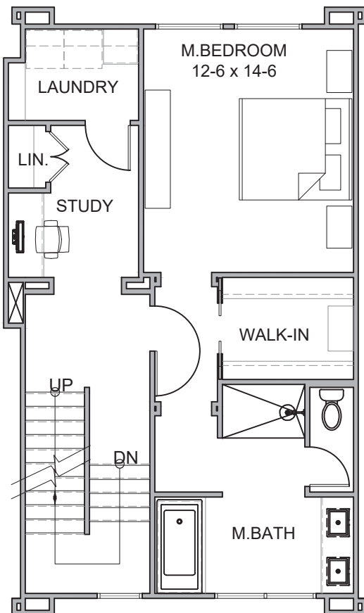
THIRD FLOOR
