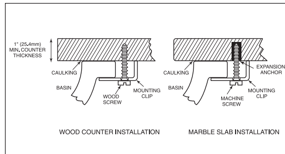
LT579G - Rendezvous Undercounter Lavatory
